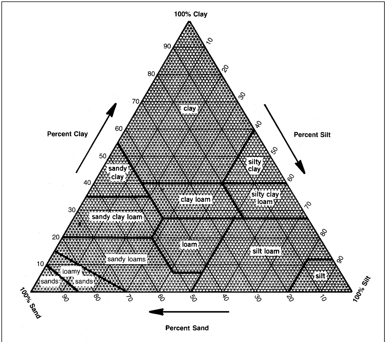
Figure 1. The USDA textural triangle, showing the twelve major textural classes in the USDA system. Within the sands, loamy sands, and sandy loams, the proportions of the various separates of sand (very coarse sand, coarse sand, medium sand, fine sand, and very fine sand) must be considered in determining which textural name to assign. If the sand fraction of a sample is dominated by a particular sand separate, a modifier must be attached to the major textural name (e.g., coarse sand, loamy very fine sand, or fine sandy loam), as discussed in the text of this fact sheet.
